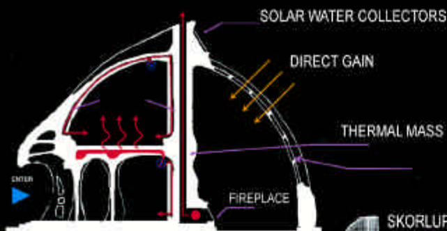
NORTH-SOUTH SECTION
